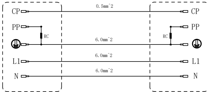
Plug wiring diagram
