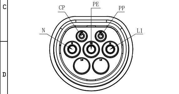
Vehicle Connector wiring diagram
