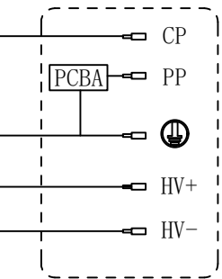
NACS Vehicle Connector wiring diagram
