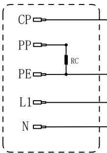
Vehicle Connector wiring diagram
