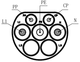
Pin Layout Chart
