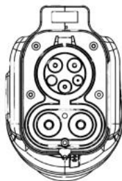
1 CCS1 Plug
